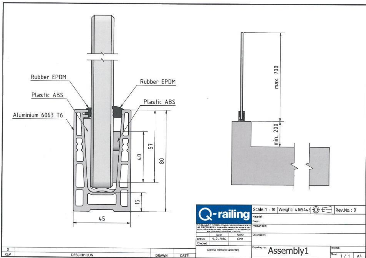
Easy Glass Up assembly drawing
